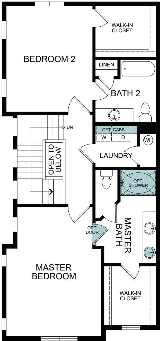
SECOND FLOOR 969 SQ. FT.
