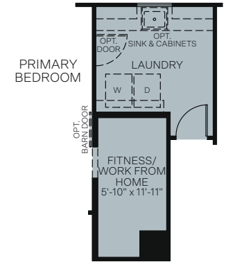
OPTIONAL LAUNDRY 2 WITH FITNESS/WORK FROM HOME
