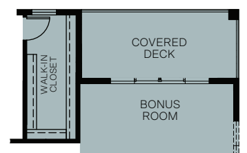
OPT. 10' SLIDER AT BONUS ROOM ILO MASTER BATH DOOR
