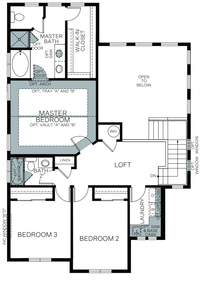
SECOND FLOOR 978 Sq. Ft.
