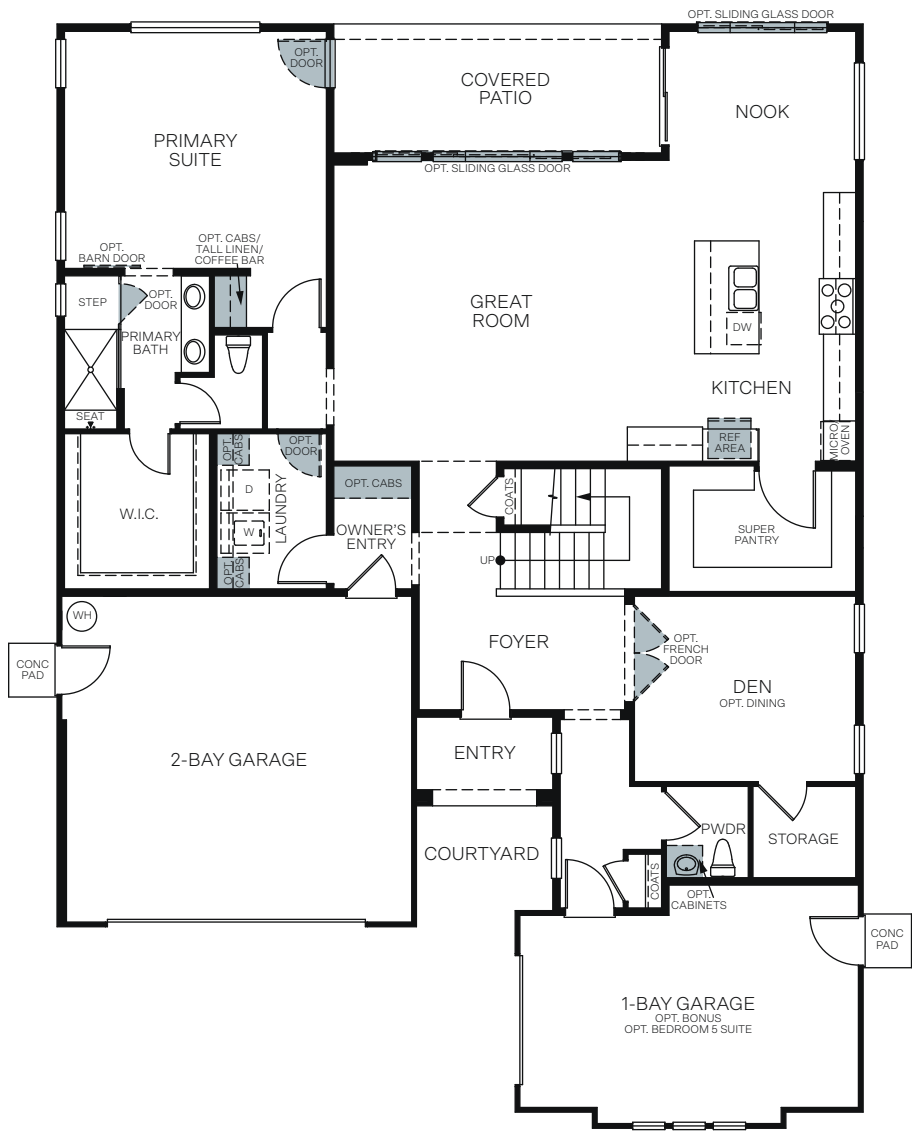
FIRST FLOOR
