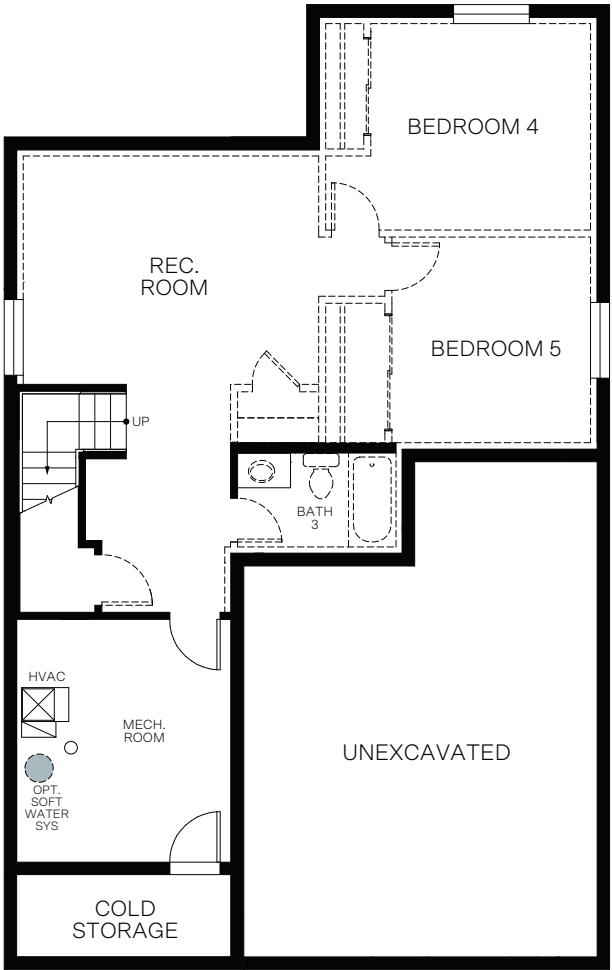
UNFINISHED BASEMENT 942 Sq. Ft.
