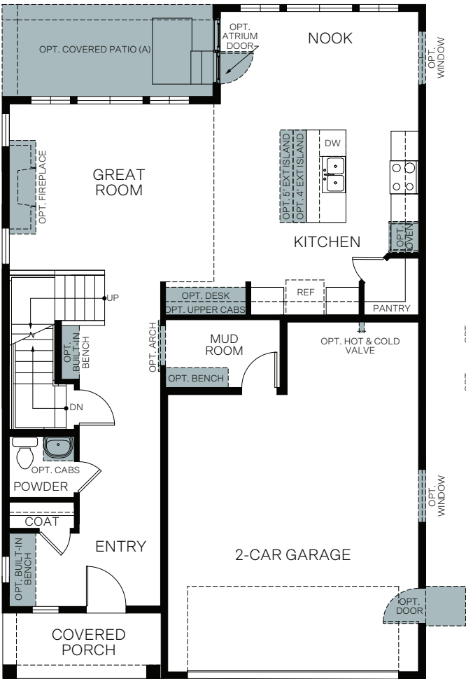
FIRST FLOOR 969 Sq. Ft.
