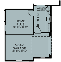
OPTIONAL HOME PLUS WITH 1-BAY GARAGE
