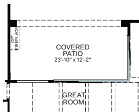
OPTIONAL CORNER MULTI-SLIDE DOOR AT GREAT ROOM
