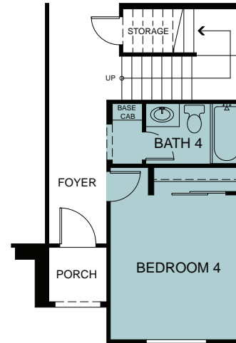
OPTIONAL BEDROOM 4 AND BATH 4 ILO FLEX AND POWDER
