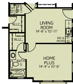
OPTIONAL HOME PLUS ILO 1-BAY GARAGE AND TEEN ROOM
