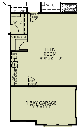
OPTIONAL TEEN ROOM EXTENSION WITH 1-BAY GARAGE ILO 1-BAY GARAGE AND TEEN ROOM
