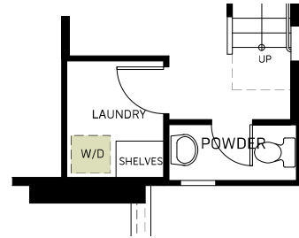
OPT. ALTERNATE LAUNDRY (TO ACCOMMODATE STACKED WASHER/DRYER)
