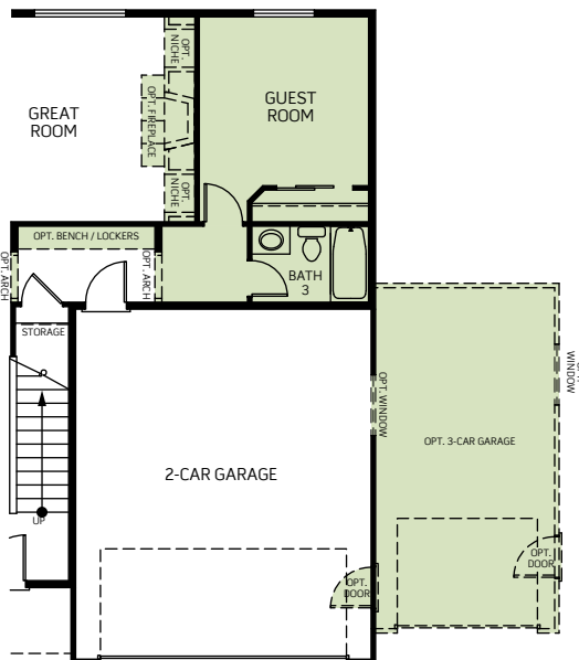
OPT. GUEST ROOM WITH BATH Adds: 210 Sq. Ft.
