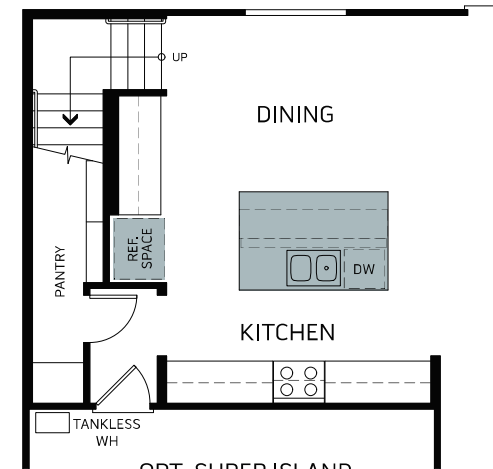
OPT. SUPER ISLAND
