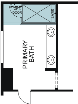
OPTIONAL WALK-IN SHOWER AT PRIMARY BATH
