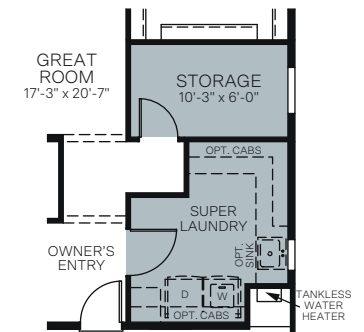
OPTIONAL SUPER LAUNDRY WITH STORAGE (NOT AVAILABLE WITH GUEST SUITE)
