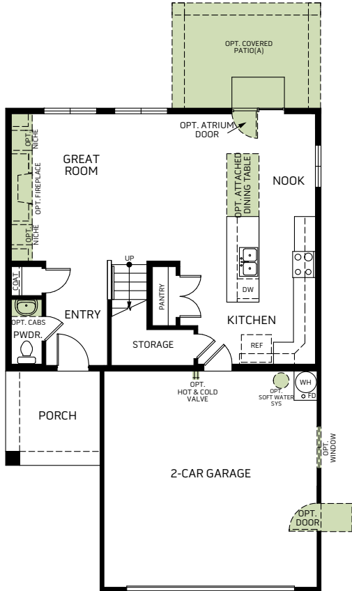
FIRST FLOOR 750 Sq.Ft.
