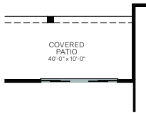
OPTIONAL 12' CENTER SLIDING GLASS DOOR AT DINING
