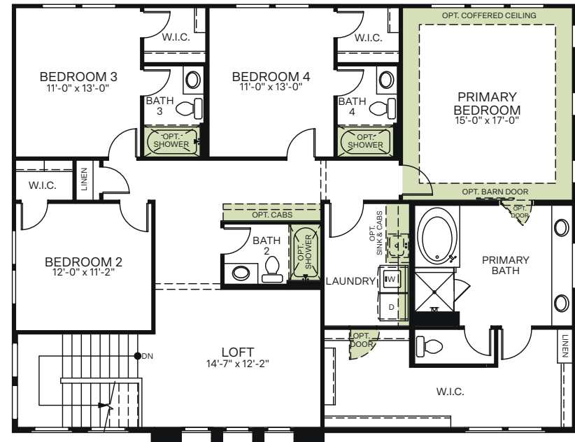
SECOND FLOOR
