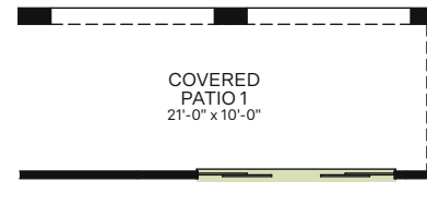
OPTIONAL 12FT. CENTER SLIDING GLASS DOOR AT GREAT ROOM
