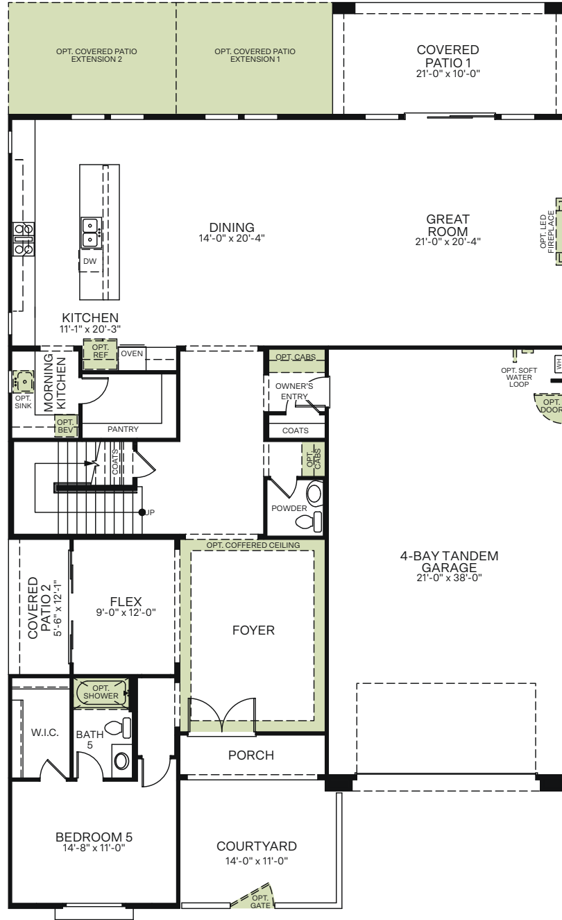
FIRST FLOOR
