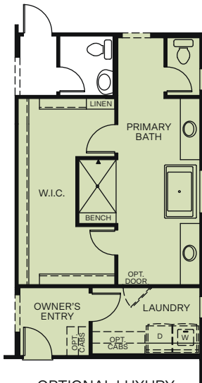
OPTIONAL LUXURY PRIMARY BATHROOM (NOT AVAILABLE WITH BONUS ROOM, WORK FROM HOME, OR SUPER LAUNDRY OPTIONS.)
