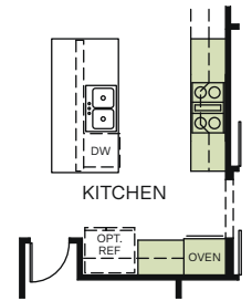
OPTIONAL KITCHEN APPLIANCE LAYOUT
