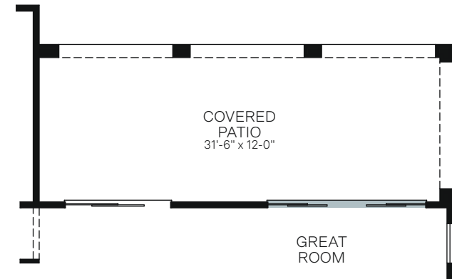
OPTIONAL 12 FT. CENTER SLIDING GLASS DOOR AT GREAT ROOM
