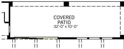
OPTIONAL 12FT MULTI-SLIDE DOOR #1 AT GREAT ROOM
