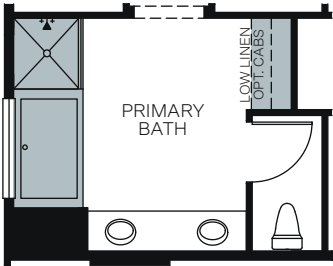
OPT. BATH/SHOWER AT PRIMARY BATH
