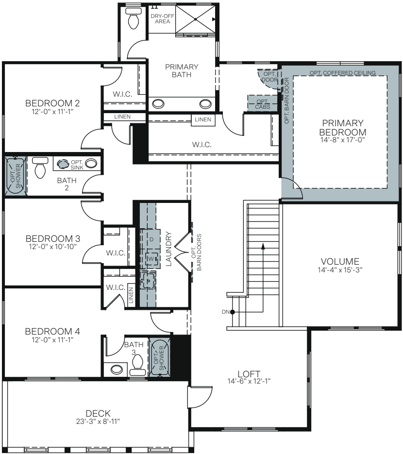
SECOND FLOOR
