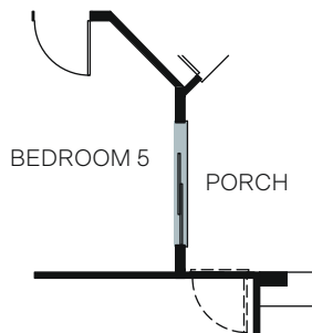
OPTIONAL 6 FT. SLIDING GLASS DOOR AT BEDROOM 5
