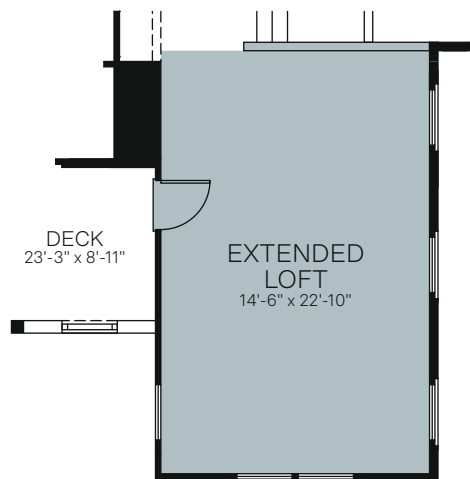
OPTIONAL EXTENDED LOFT (NOT AVAILABLE WITH BEDROOM 7)
