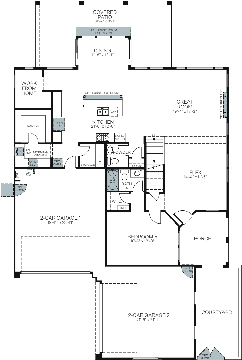
FIRST FLOOR
