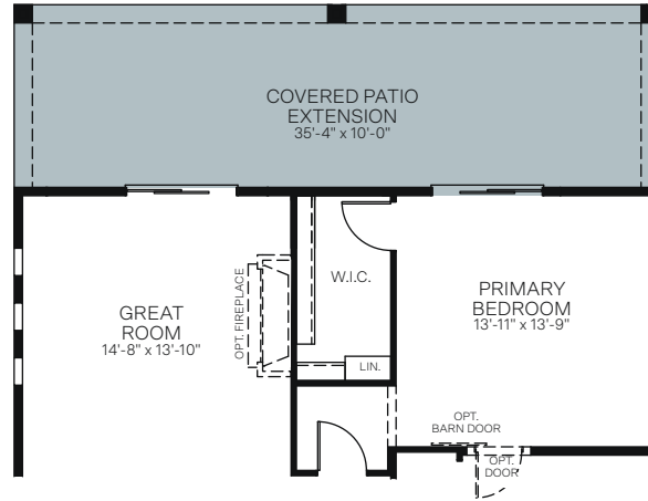
OPTIONAL 6 Ft. SLIDING GLASS DOOR AT PRIMARY BEDROOM (ONLY AVAILABLE WITH COVERED PATIO EXTENSION)
