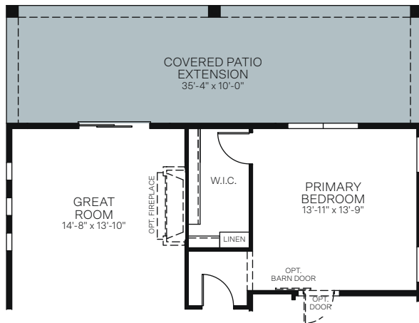
OPTIONAL COVERED PATIO EXTENSION
