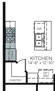
OPTIONAL KITCHEN APPLIANCE LAYOUT
