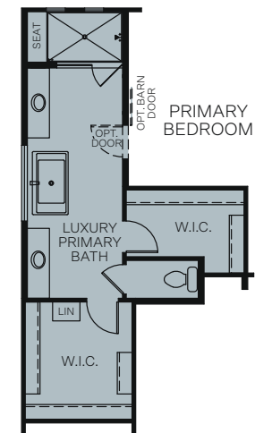
OPTIONAL LUXURY PRIMARY BATHROOM (NOT AVAILABLE WITH FITNESS/WORK FROM HOME OPTION)
