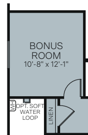
OPTIONAL BONUS ROOM ILO TANDEM GARAGE
