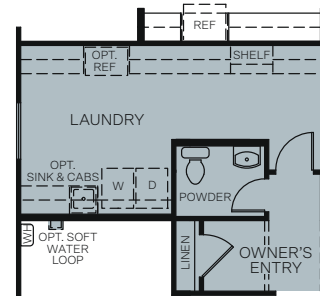
OPTIONAL SUPER LAUNDRY 2 (NOT AVAILABLE WITH LUXURY PRIMARY BATH, BONUS, OR STORAGE ROOM OPTIONS)
