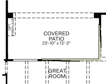
OPTIONAL CORNER MULTI-SLIDE DOOR AT GREAT ROOM
