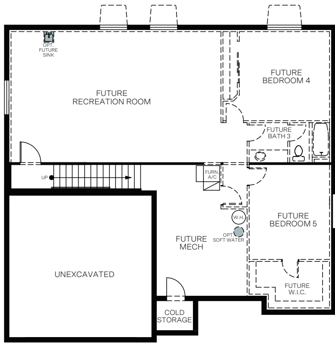
BASEMENT PLAN 1,523 Sq. Ft.
