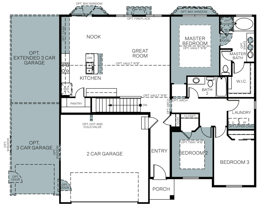
FLOOR PLAN 1,558 Sq. Ft.
