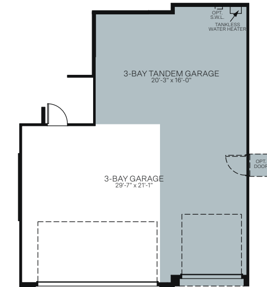
OPTIONAL 3-BAY TANDEM GARAGE (LENGTH OF 3-BAY GARAGE DOES NOT EXTEND WITH 2'-0" AND 4'-0" GARAGE EXTENSIONS)
