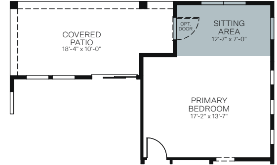
OPTIONAL SITTING AREA AT PRIMARY BEDROOM (NOT AVAILABLE WITH BAY WINDOW AT PRIMARY BEDROOM) (NOT AVAILABLE WITH COVERED PATIO EXTENSION) (NOT AVAILABLE WITH 8 FT. SLIDING GLASS DOOR AT PRIMARY BEDROOM)
