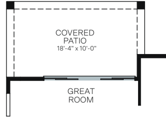
OPTIONAL 12 Ft. CENTER SLIDING GLASS DOOR AT GREAT ROOM
