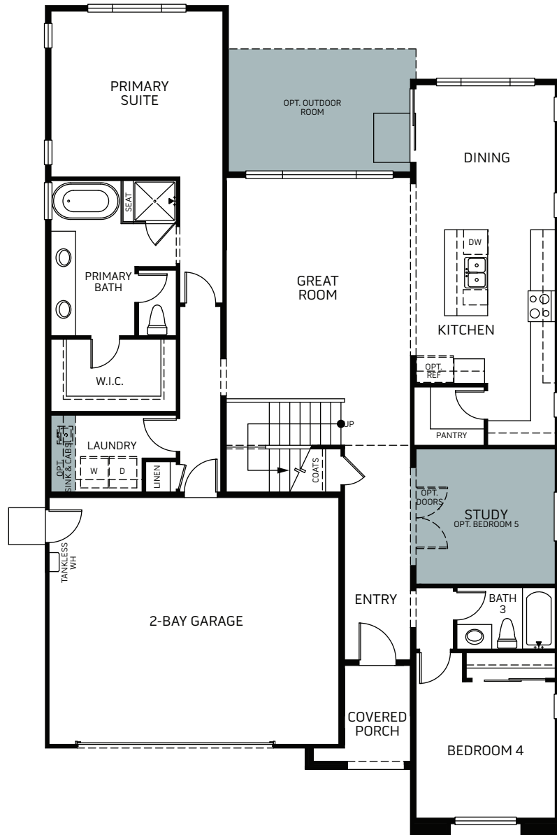
FIRST FLOOR
