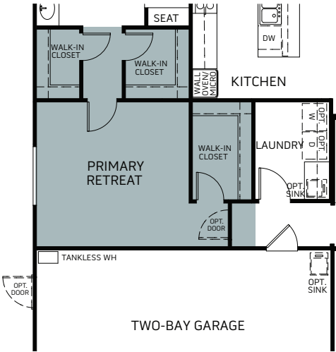
OPT. PRIMARY RETREAT ILO BEDROOM 3 and BATH 3
