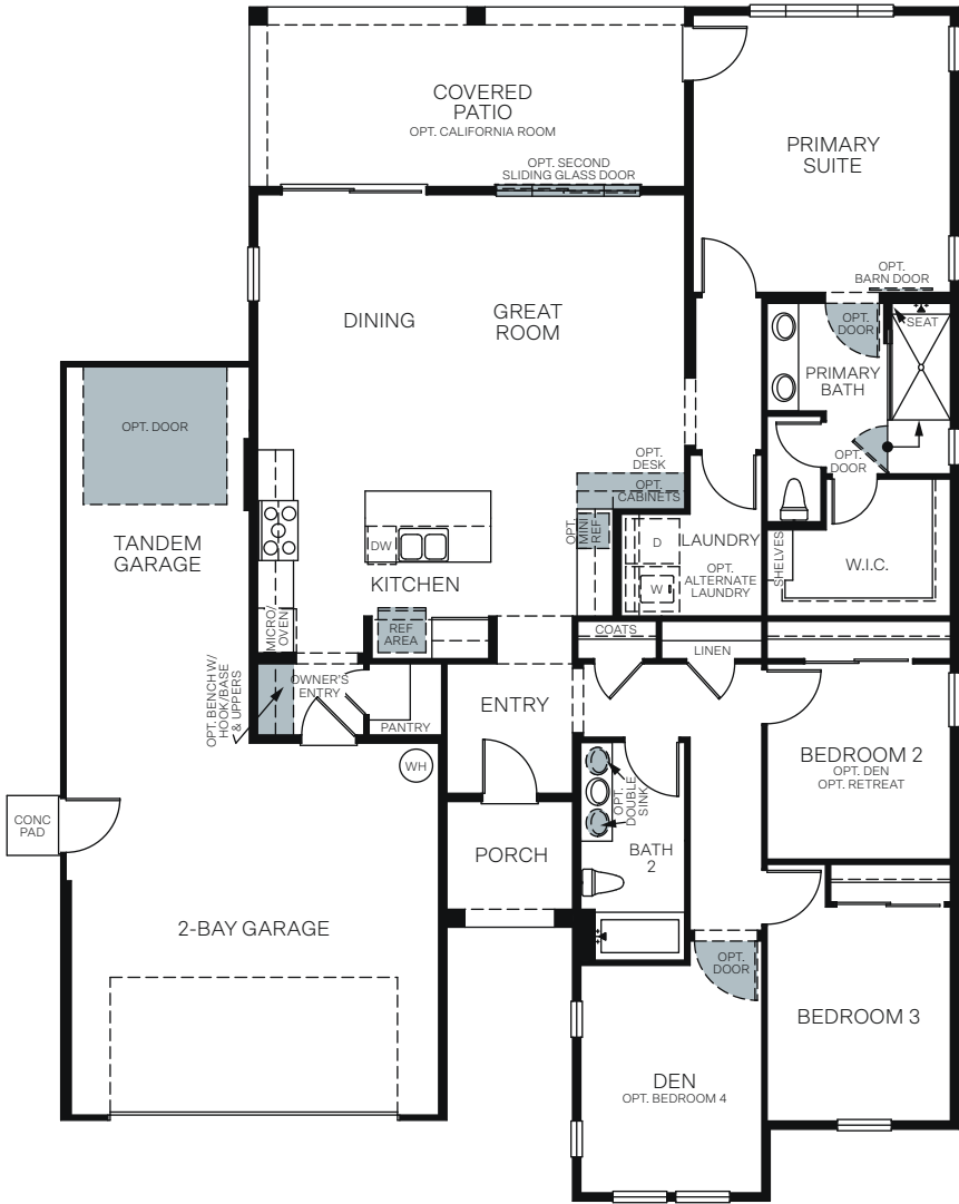
FLOOR PLAN
