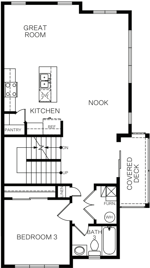
SECOND FLOOR 860 Sq. Ft.
