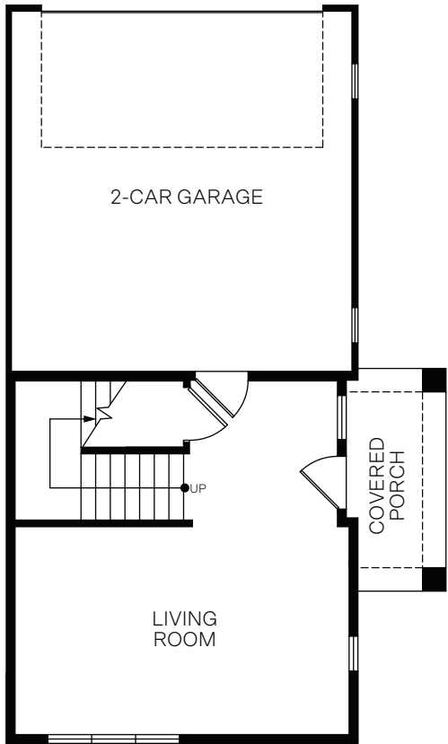
FIRST FLOOR 389 Sq. Ft.
