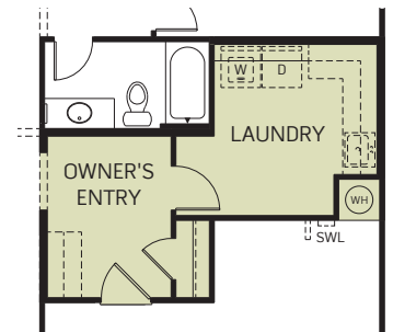
OPTIONAL SUPER LAUNDRY 1 ILO TANDEM
