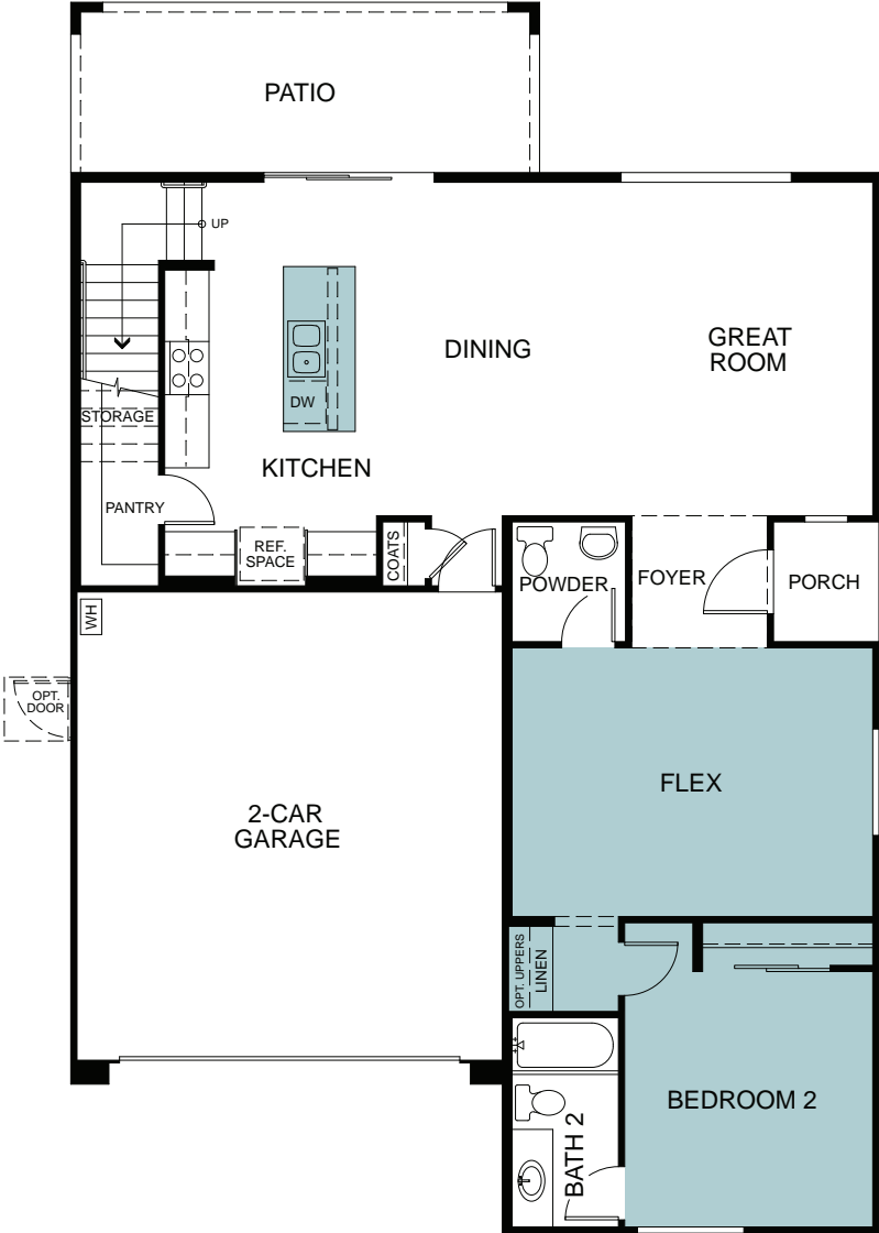
FIRST FLOOR
