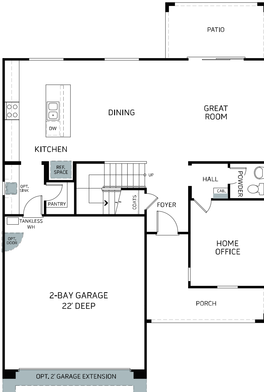
FIRST FLOOR
