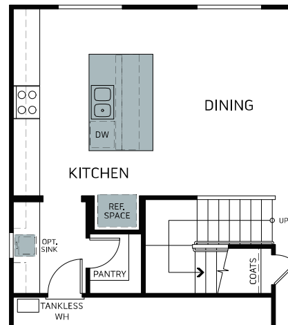
OPT. SUPER ISLAND
