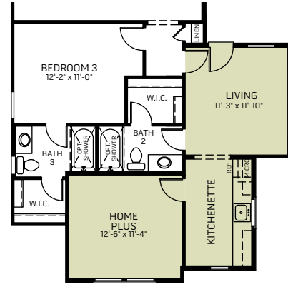
OPTIONAL HOME PLUS ILO 1-BAY GARAGE (not available with 2-bay garage) (not available with home plus with 1-bay garage)
