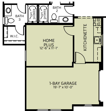
OPTIONAL HOME PLUS WITH 1 BAY GARAGE ILO 1-BAY GARAGE (not available with 2-bay garage) (not available with home plus)
