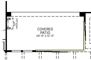
OPTIONAL CORNER MULTI SLIDE DOORS
