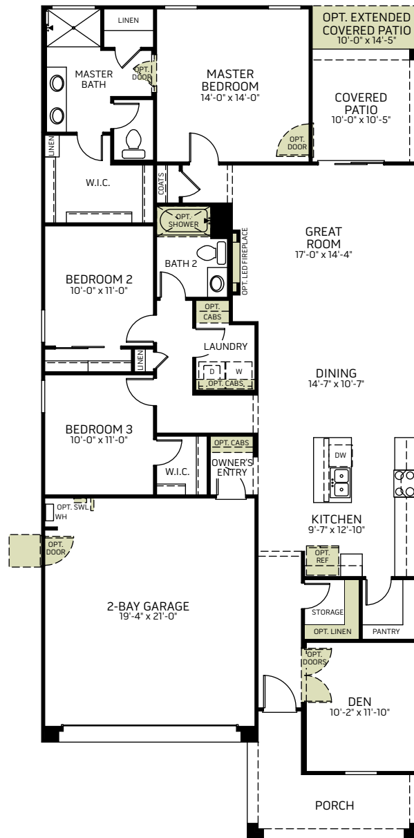
FLOOR PLAN
