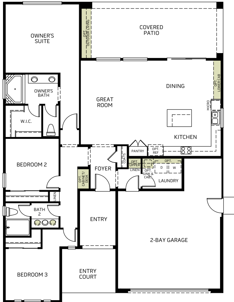
FLOOR PLAN
