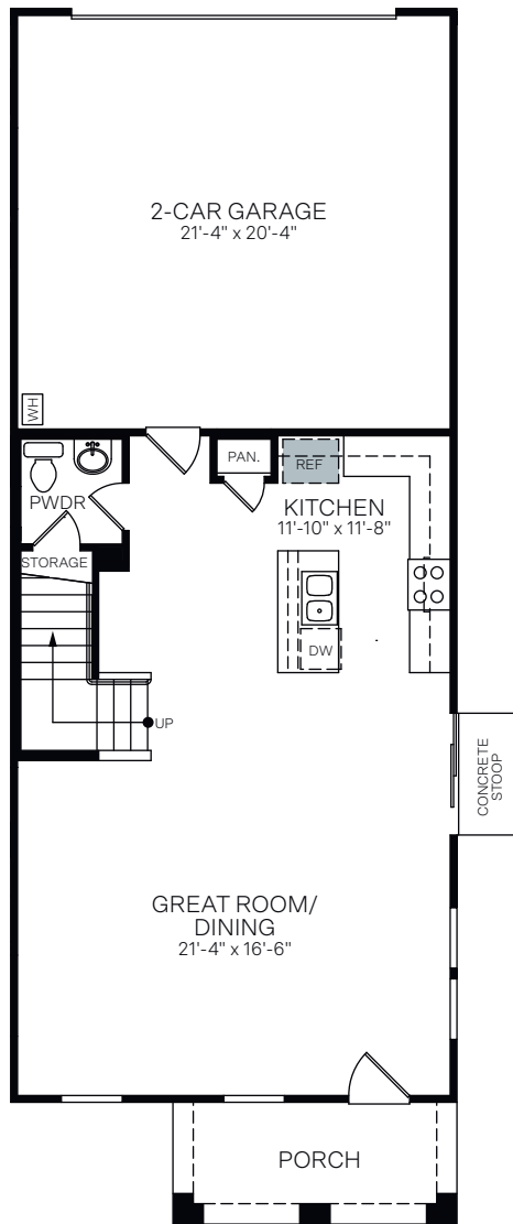
FIRST FLOOR
