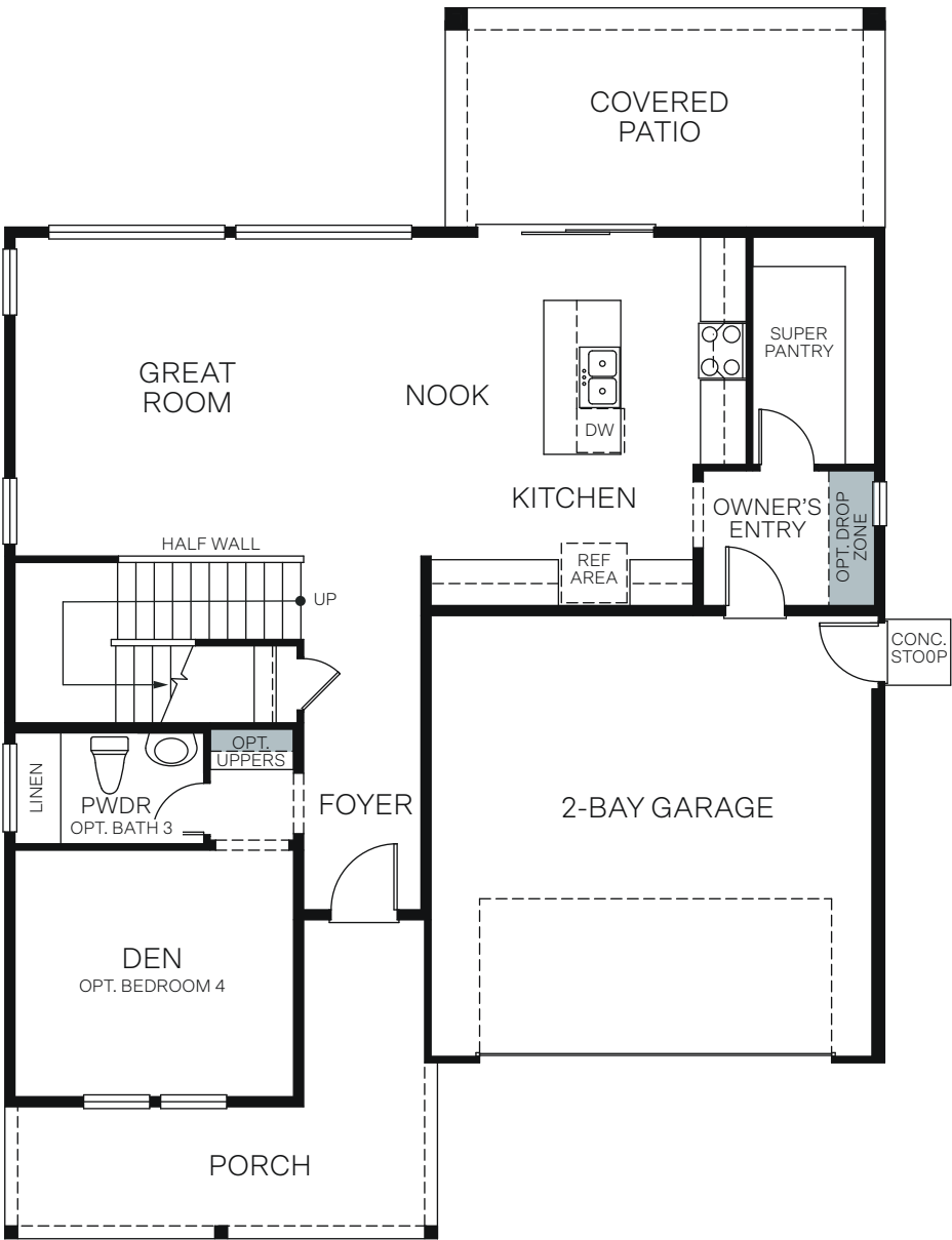
FIRST FLOOR
