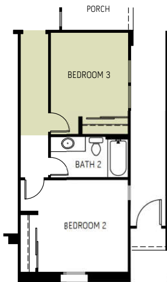
OPT. BEDROOM 3 ILO FLEX
