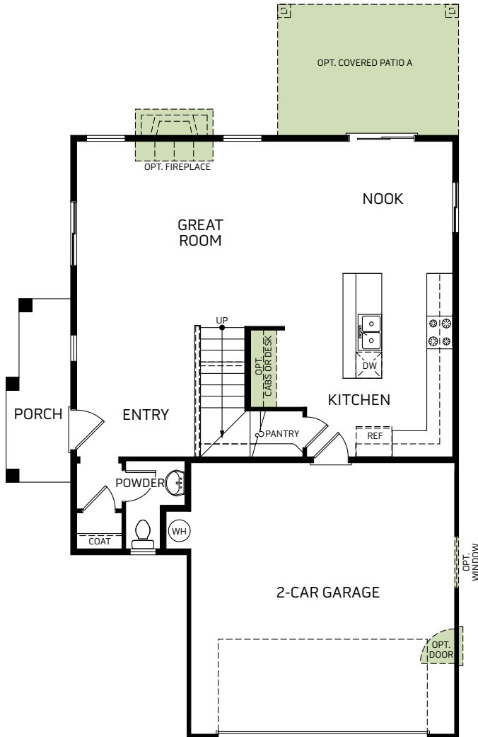
FIRST FLOOR PLAN 807 Sq. Ft.
