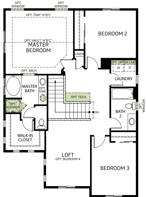
SECOND FLOOR PLAN 1,095 Sq. Ft.
