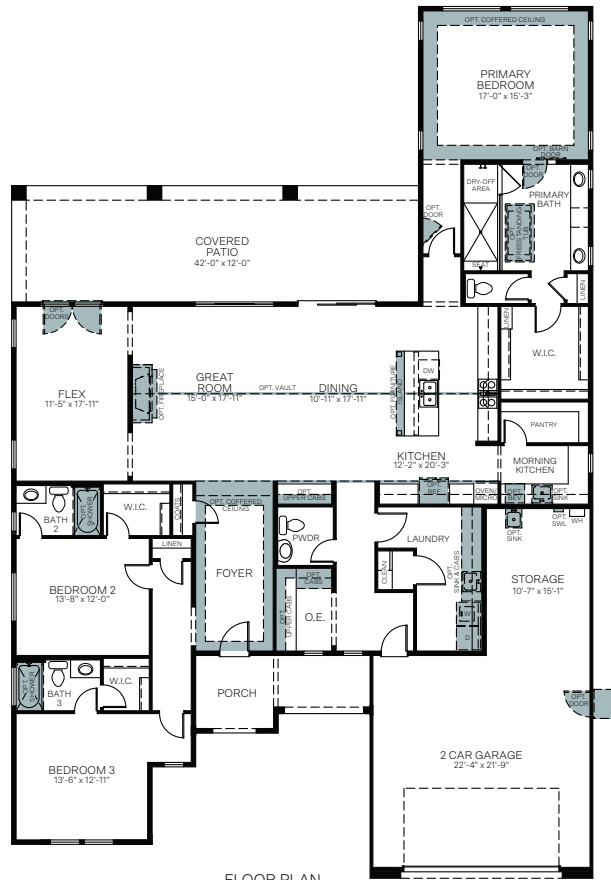
FLOOR PLAN 2,907 Sq.Ft.
