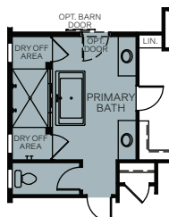
OPTIONAL FREESTANDING TUB AT PRIMARY BATHROOM
