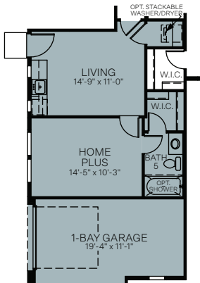
OPTIONAL HOME PLUS W/ 1-BAY GARAGE ILO 1-BAY GARAGE AND TEEN ROOM (NOT AVAILABLE WITH HOME PLUS OPTIONS) (NOT AVAILABLE WITH 2-BAY GARAGE OPTIONS) (NOT AVAILABLE WITH MEDIA/BEDROOM 5 OPTIONS)
