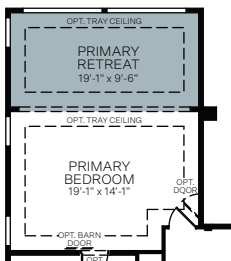
OPTIONAL PRIMARY RETREAT
