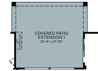
OPTIONAL COVERED PATIO EXTENSION 1
