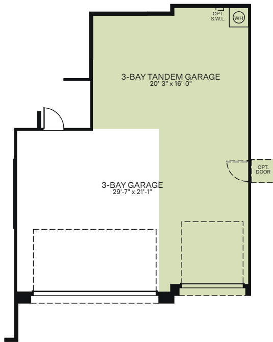
OPTIONAL 3-BAY TANDEM GARAGE (LENGTH OF 3-BAY GARAGE DOES NOT EXTEND WITH 2'-0" AND 4'-0" GARAGE EXTENSIONS)
