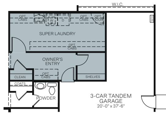
OPTIONAL SUPER LAUNDRY
