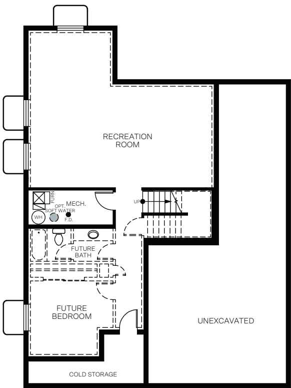
BASEMENT 1,026 Sq.Ft.
