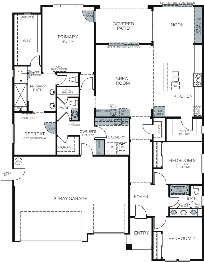
FLOOR PLAN
