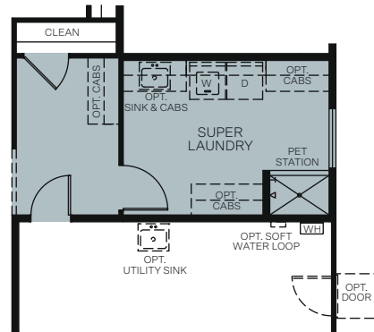
OPTIONAL SUPER LAUNDRY WITH PET STATION (NOT AVAILABLE WITH BONUS ROOM OPTION)
