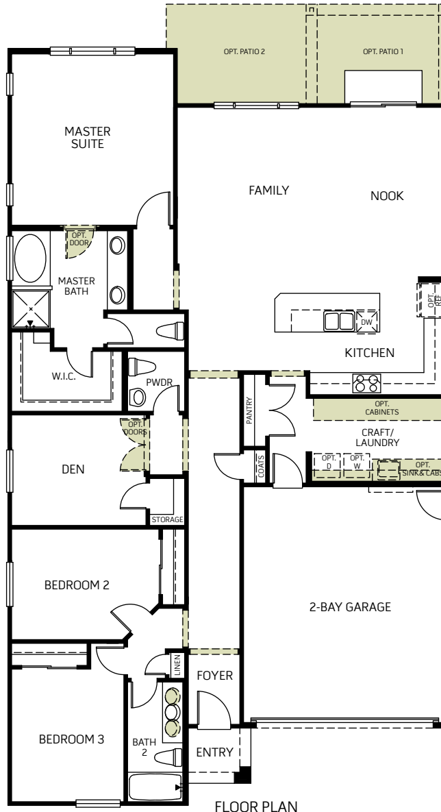
FLOOR PLAN
