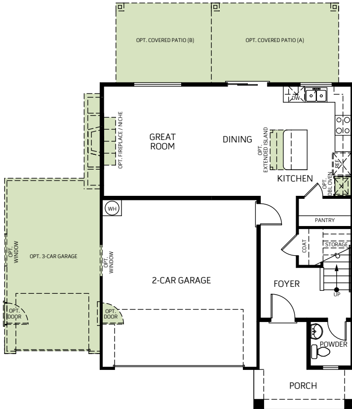
FIRST FLOOR 695 Sq. Ft.
