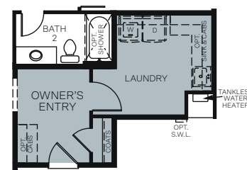
OPTIONAL SUPER LAUNDRY 1 ILO TANDEM (NOT AVAILABLE WITH SUPER LAUNDRY 2, FLEX, 4-BAY GARAGE)
